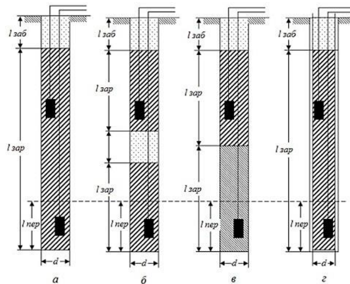
Figure 1. Various designs of borehole charges: a — solid charge column; b — charge column dispersed with an inert spacer; c — combined charge of different types of explosives; d — charge in a sleeve.
